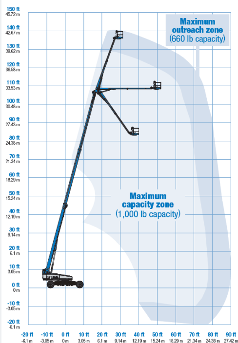
Range Of Motion SX-135 XC
